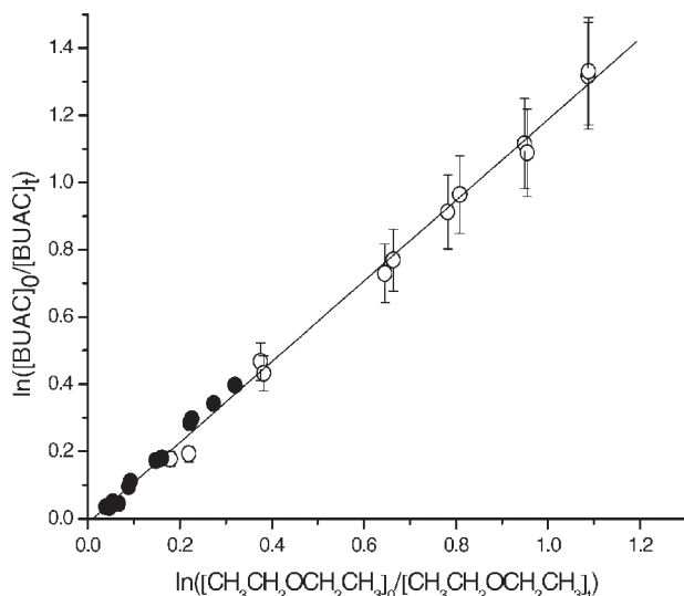
Figure 2. Relative rate data for the OH reaction with butyl acrylate using diethyl ether as reference compound at 298 K and atmospheric pressure of N 2 (○) and air (●)
