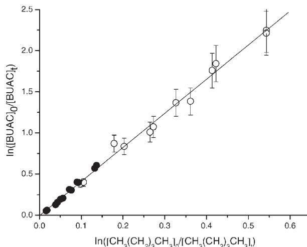
Figure 3. Relative rate data for the OH reaction with butyl acrylate using n -pentane as reference compound at 298 K and atmospheric pressure of N 2 (○) and air (●)
