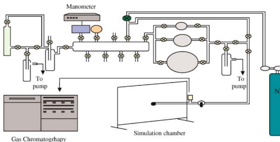
Figure 1. Schematic diagram of the simulation chamber apparatus used in the OH + BUAC reaction study
